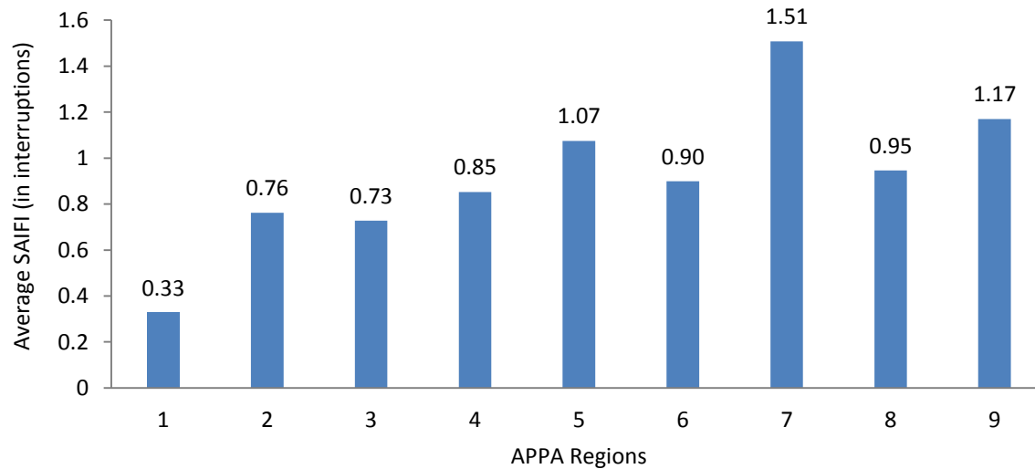
Figure 9: Average SAIFI by APPA region
