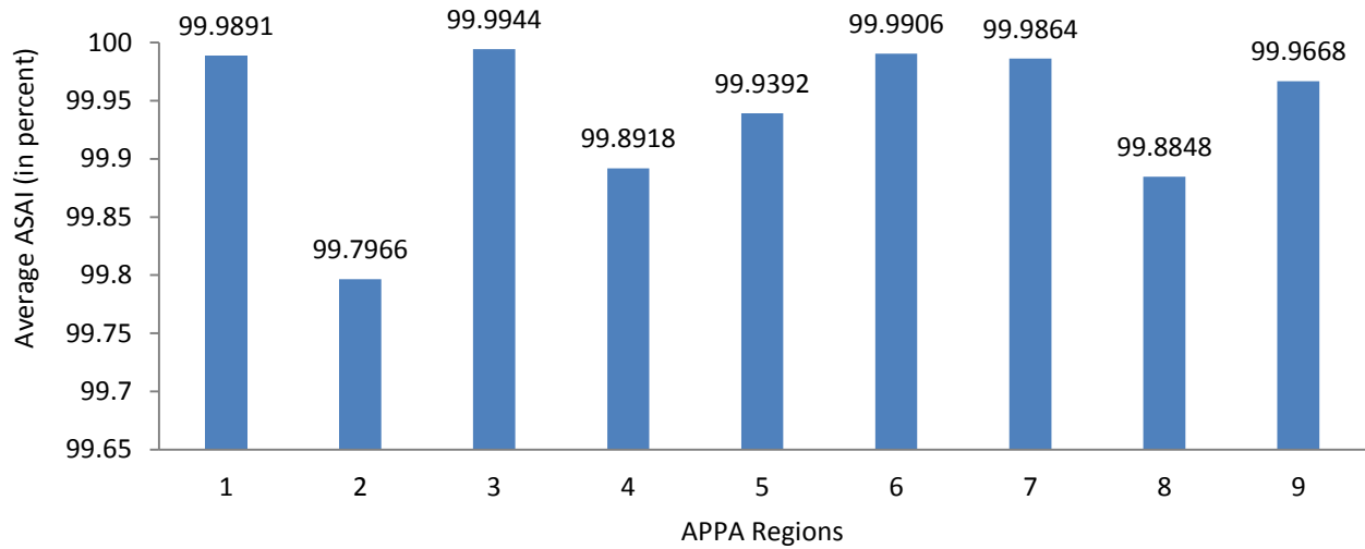
Figure 12: Average ASAI by APPA region
