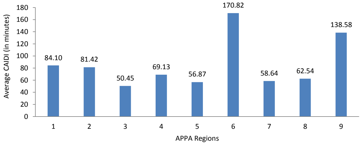
Figure 11: Average CAIDI by APPA region
